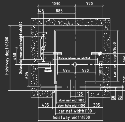
Hoistway plane layout
