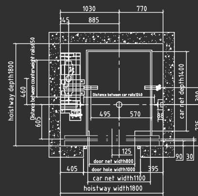
Hoistway top plane layout
