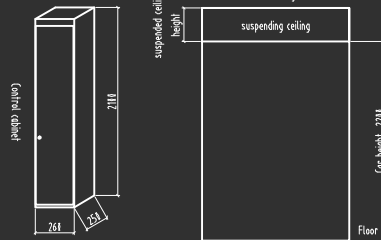
Size of the control cabinet
