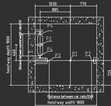
Pit plane layout
